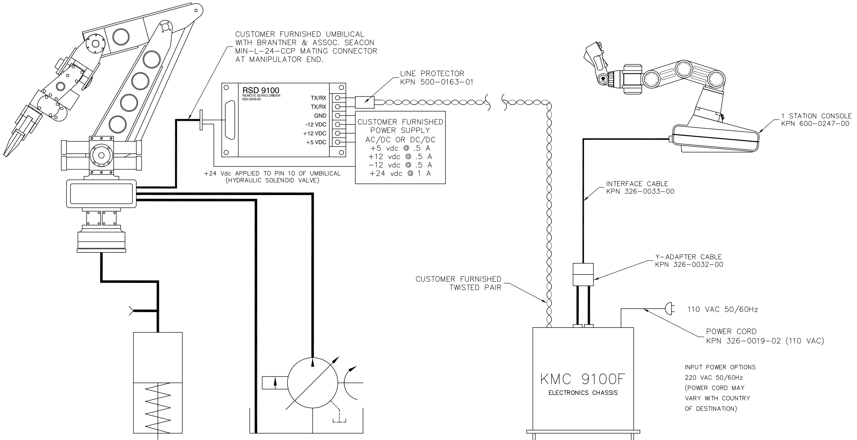
CUSTOMER FURNISHED POSITIVE COMPENSATOR UNIT (REQUIRED FOR UNDERWATER USE ONLY)
